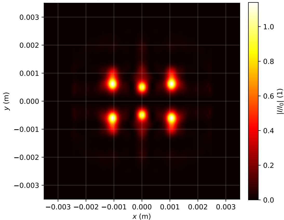
Intensity profile I(x, y, z = 2.070)/I_0 , P_{in}=6.0P_{cr} , artificial time
